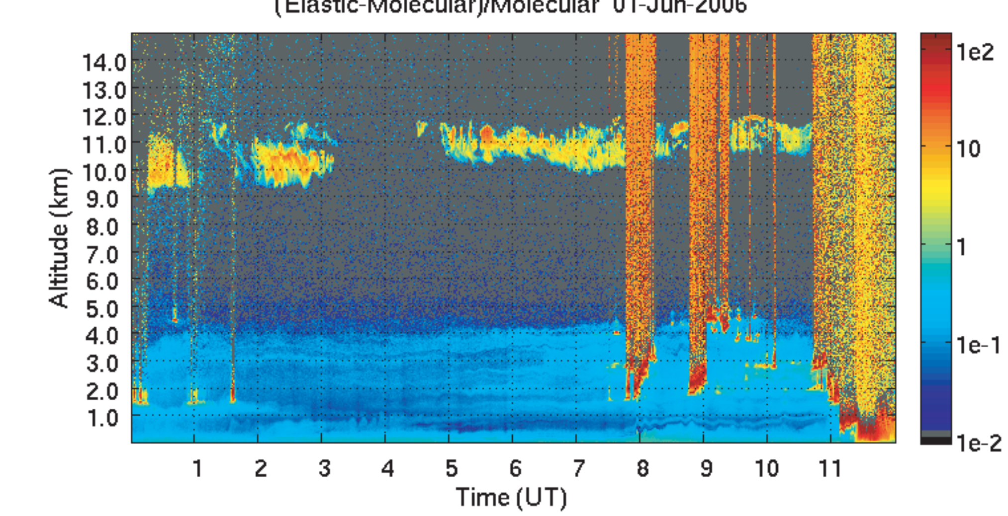
An example of the backscatter cross section measured by the Raman system at the CART site in Oklahoma. Here shown uncalibrated.
