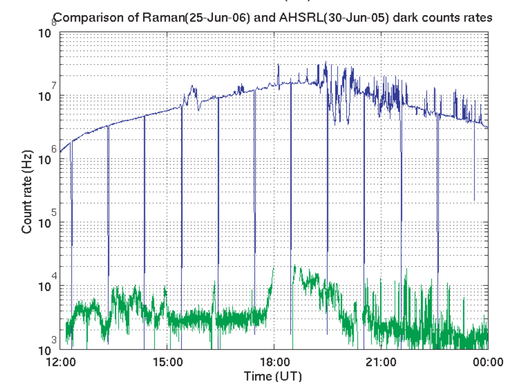
Background noise counts and count rates observed with the AHSRL and Raman systems.
