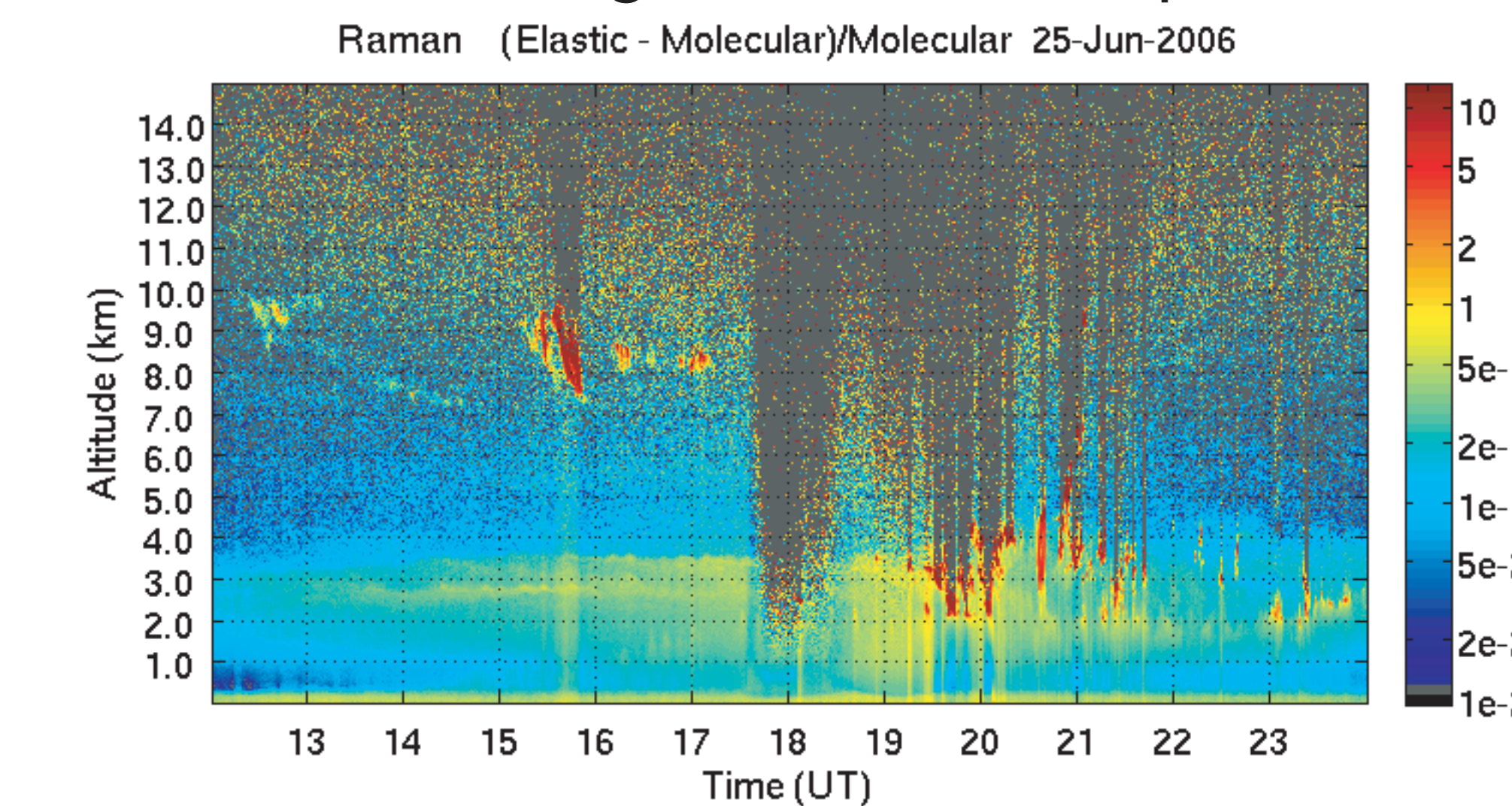
Raman observed aerosol returns in the case used for noise comparisons.
