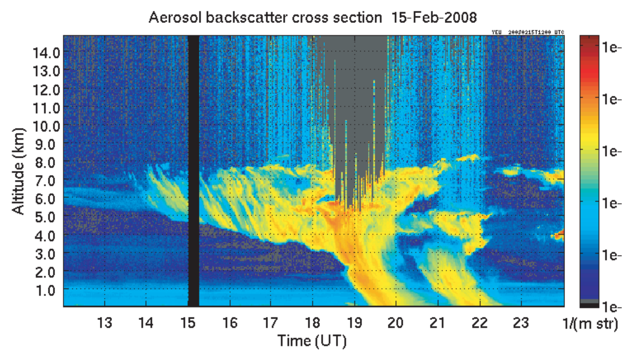
A example of the backscatter cross section measured by the AHSRL in Eureka, Canada
