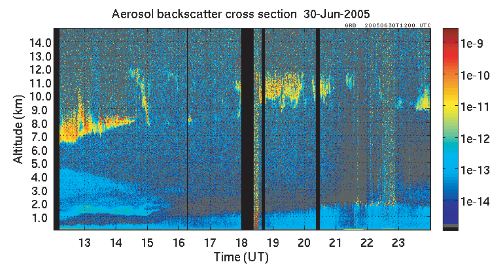
AHSRL observed backscatter cross section in the case used for background noise comparisons.
